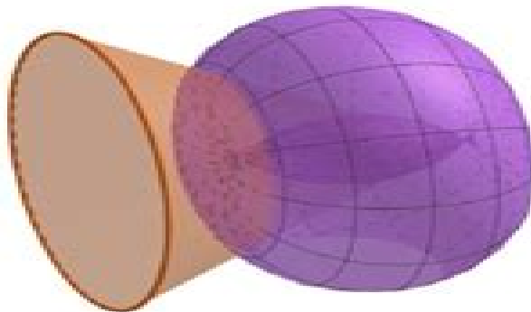
FIGURE 4. The intersection of a cone and spindle torus that share the same axis is a circle.
