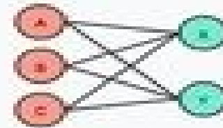
Bipartite Graph
